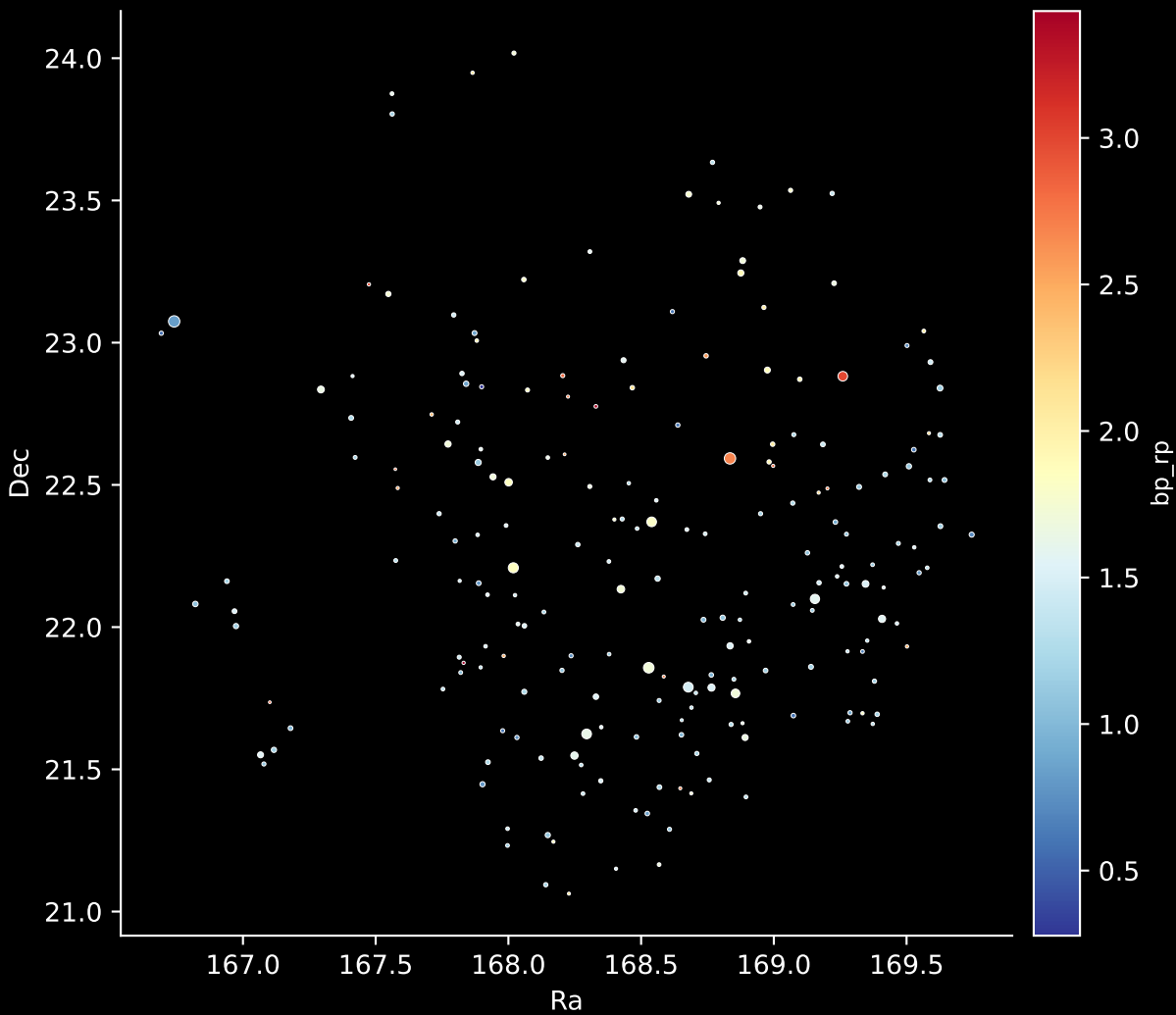
APOGEE DR17 Field: [K2_C13_176-17_btx] Stars: 206
