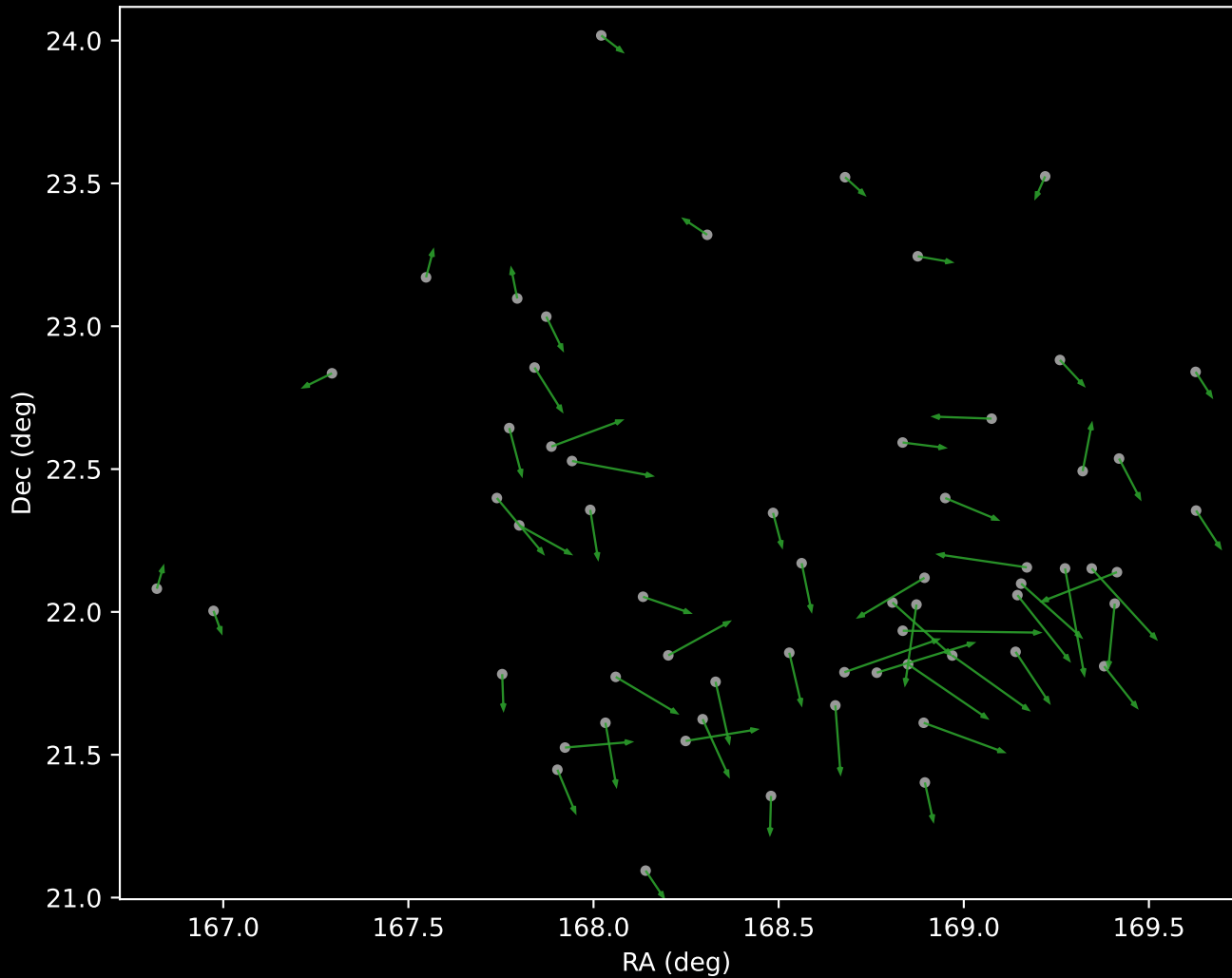
APOGEE DR17 Cluster 4 Proper Motion Vectors (n=61)
