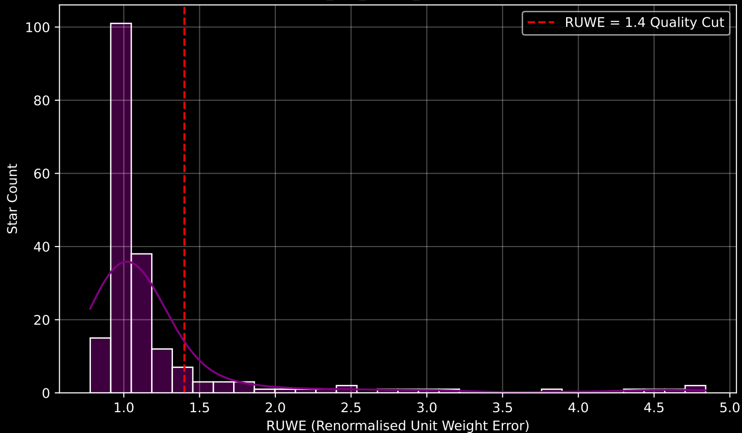
GAPOGEE DR17 Field [K2_C13_176-17_btx] RUWE Distribution (n= 198)
