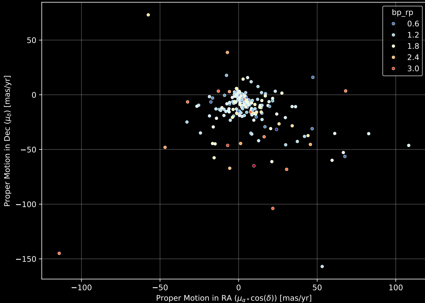
APOGEE DR17 Field: [K2_C13_176-17_btx] Proper Motion Diagram (n= 206)
