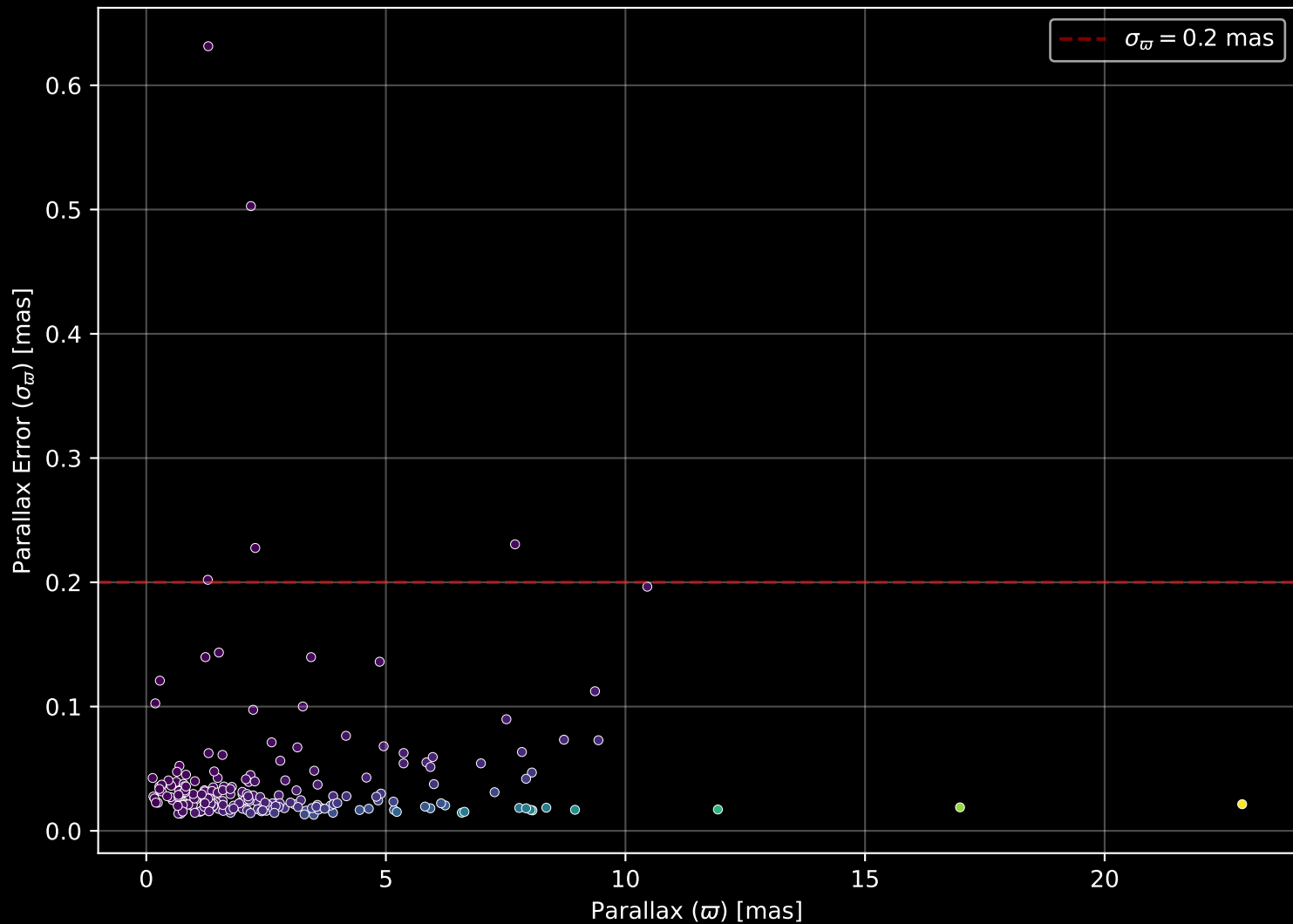
APOGEE DR17 Field: [K2_C13_176-17_btx] Parallax Quality (n= 206)
