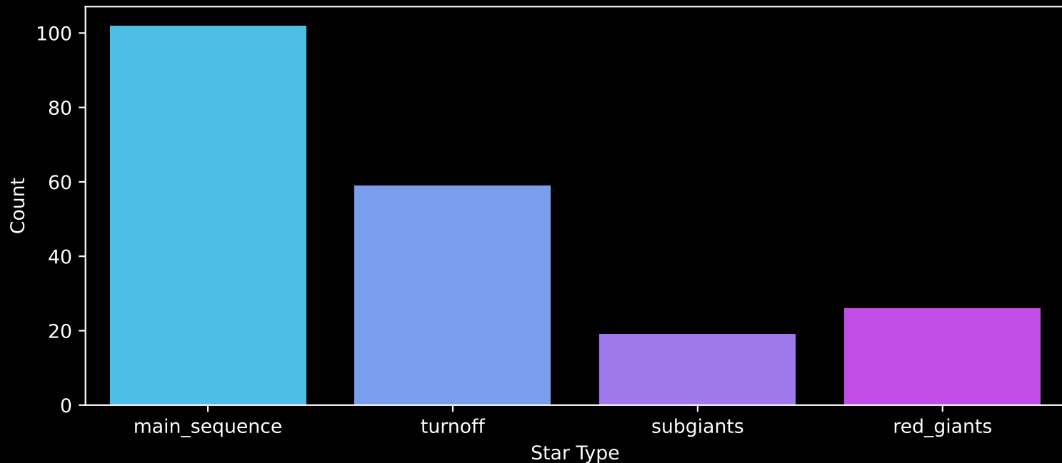
APOGEE DR17 Field: [K2_C13_176-17_btx] Count plot of Star Type
