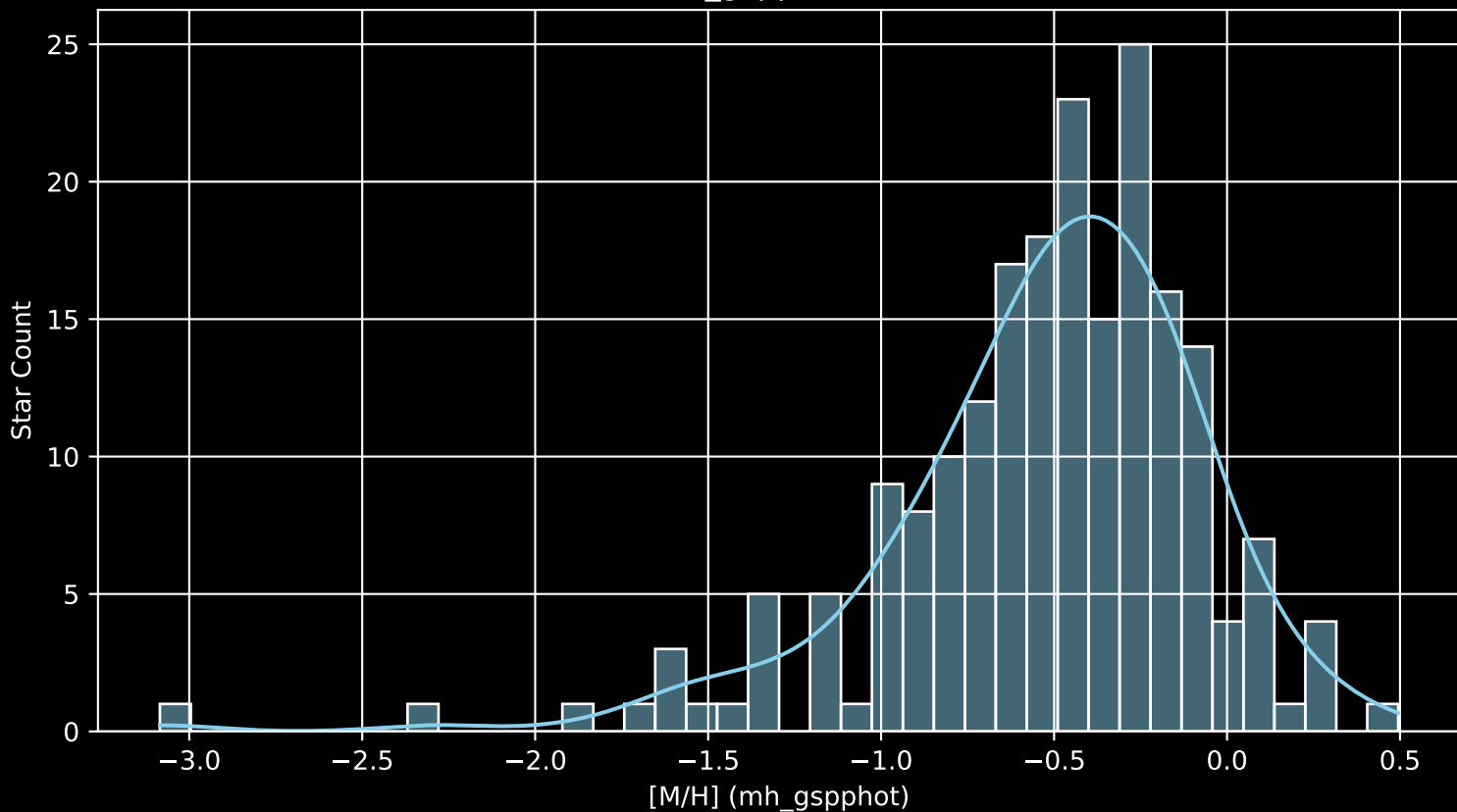
APOGEE DR17 Field: [K2_C13_176-17_btx [M/H] (mh_gspphot) (n= 204)
